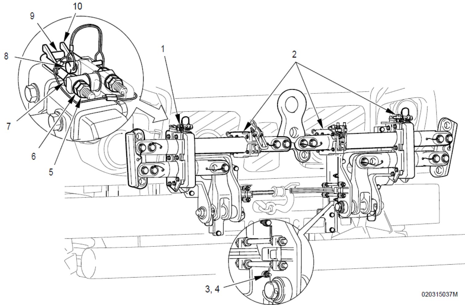
Figure 7. Towbar Secured.
